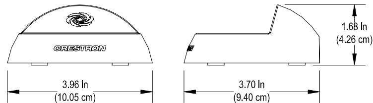
CEN-IDOCV-DS Dimensions
