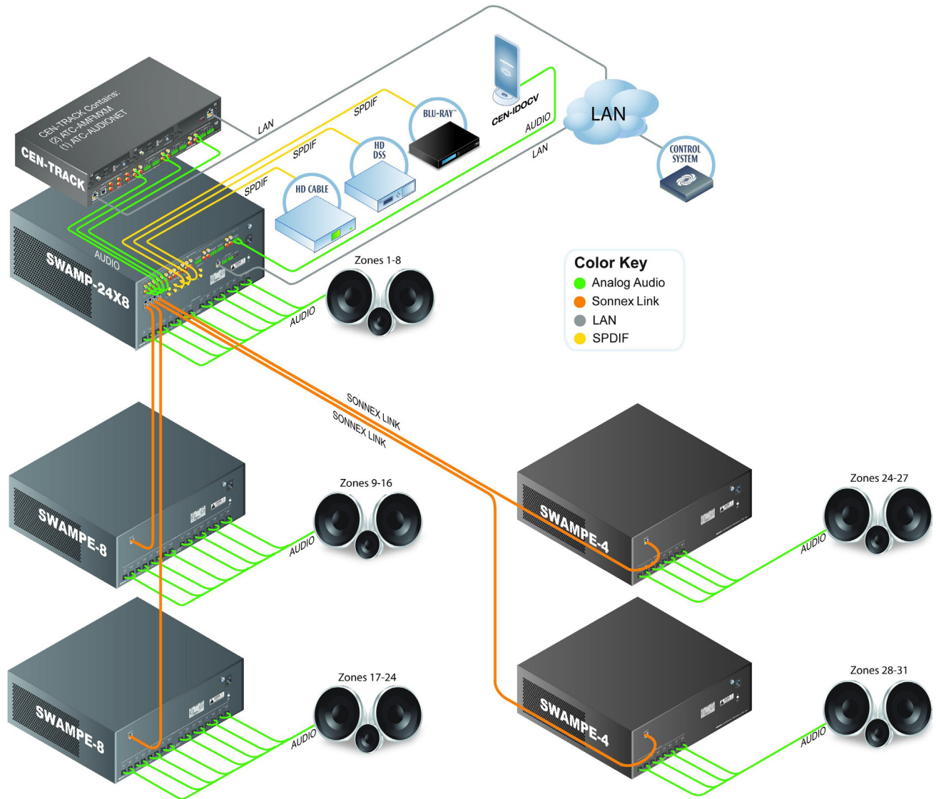
SWAMPE-8 in a Multizone Application
