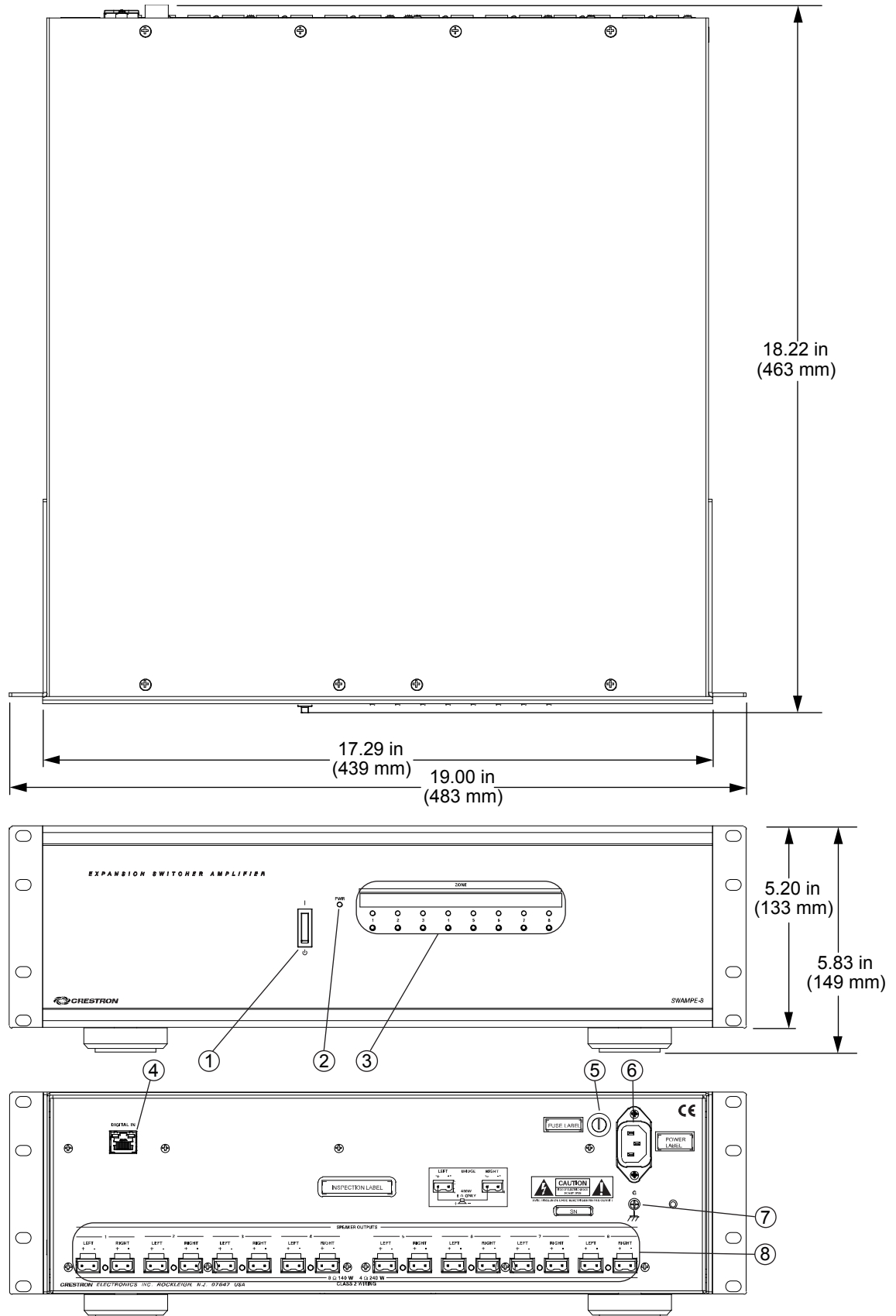
SWAMPE-8 Overall Dimensions
