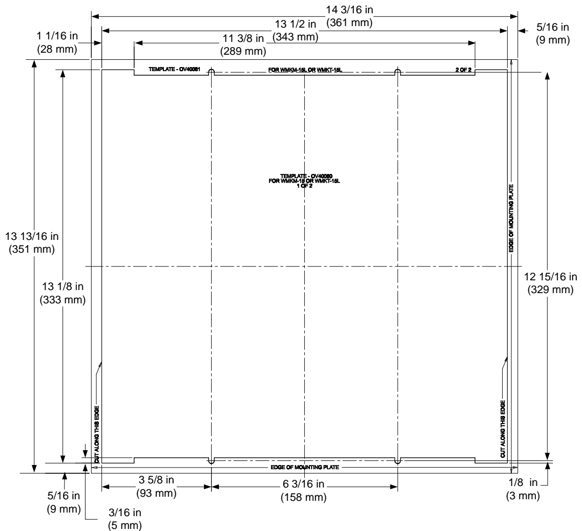
Drywall Cutout Template and Dimensions (supplied with WMKT-15L only)
