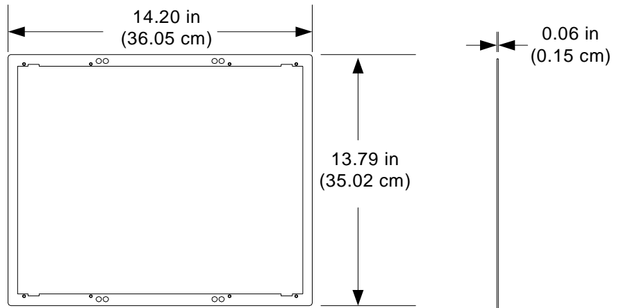
Dimensional Drawing – Mounting Plate
