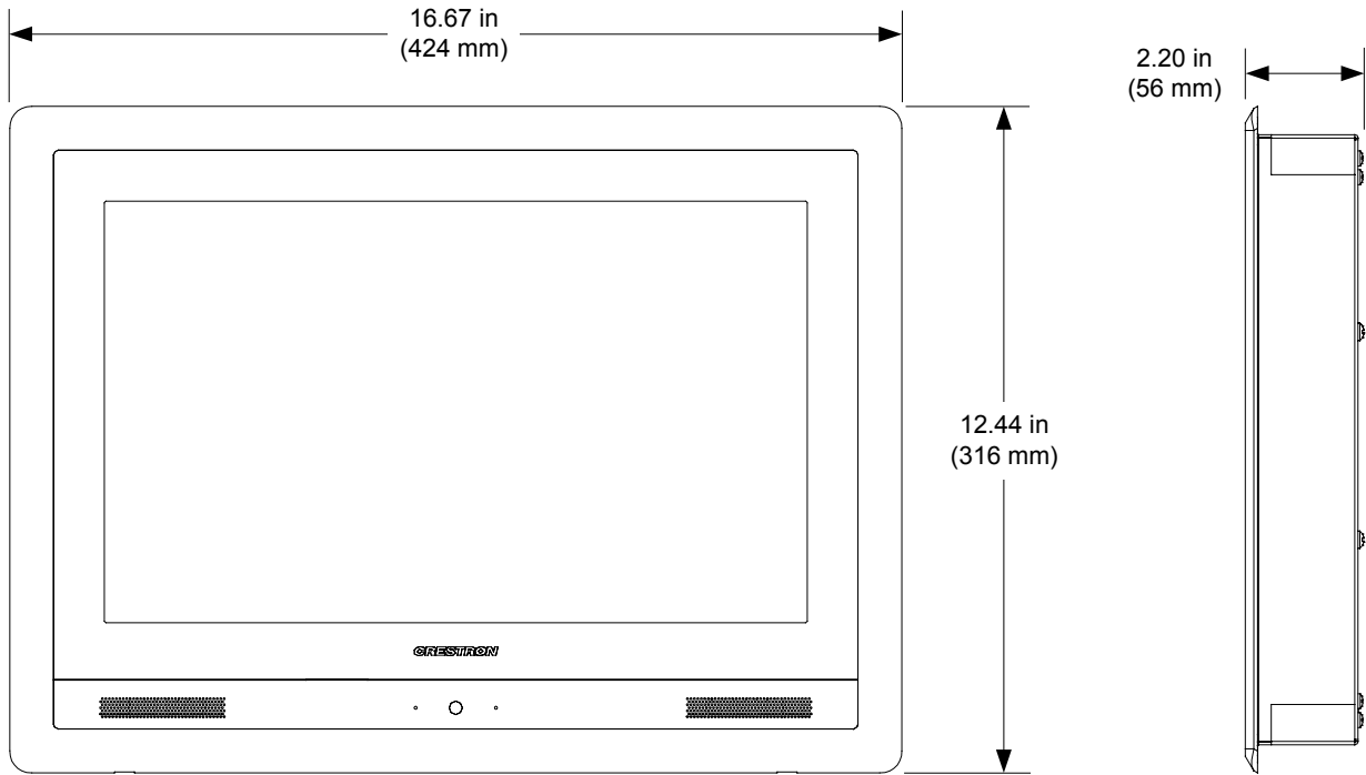
TPMC-V15-WALL and V15-WALL Overall Dimensions (Front and Side Views - With Bezel)
