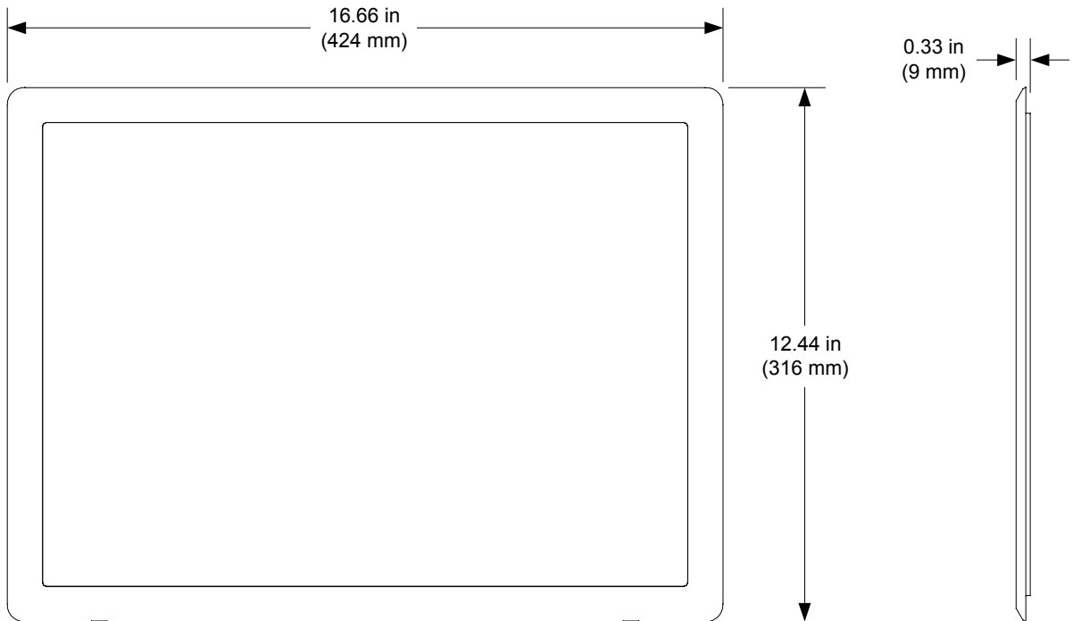
Bezel Overall Dimensions (Front and Side Views)
