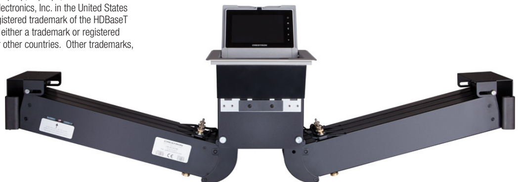
FT-TS600 with CBLR Cable Retractors in Horizontal Orientation
