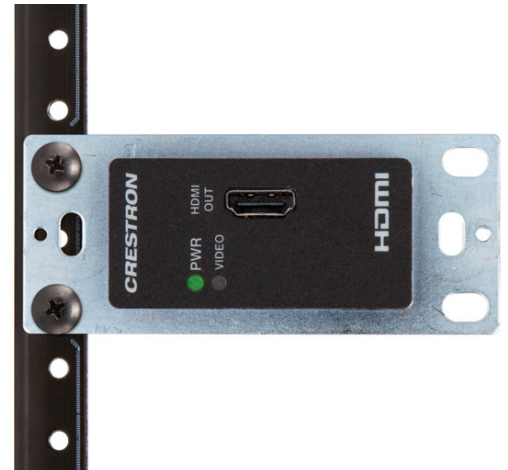
DM-RX1-4K-C-1G-B-T – Attached to Rack Rail
