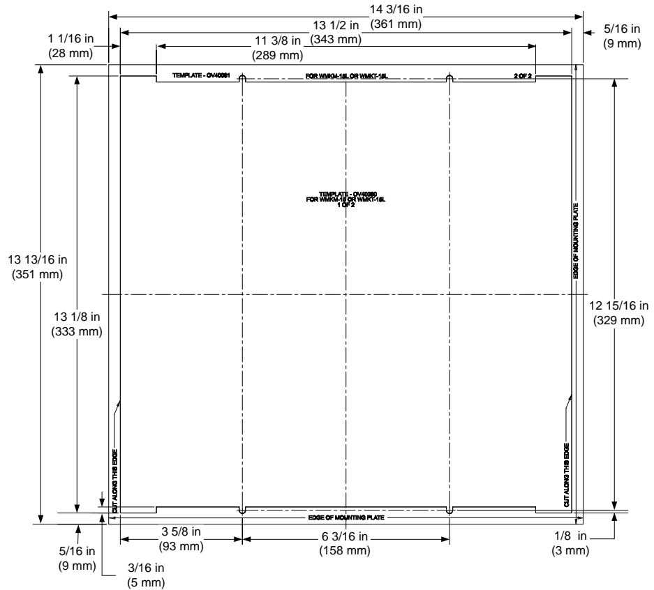
Drywall Cutout Template and Dimensions (supplied with WMKM-15L only)
