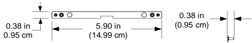
Dimensional Drawing – Mounting Plate
