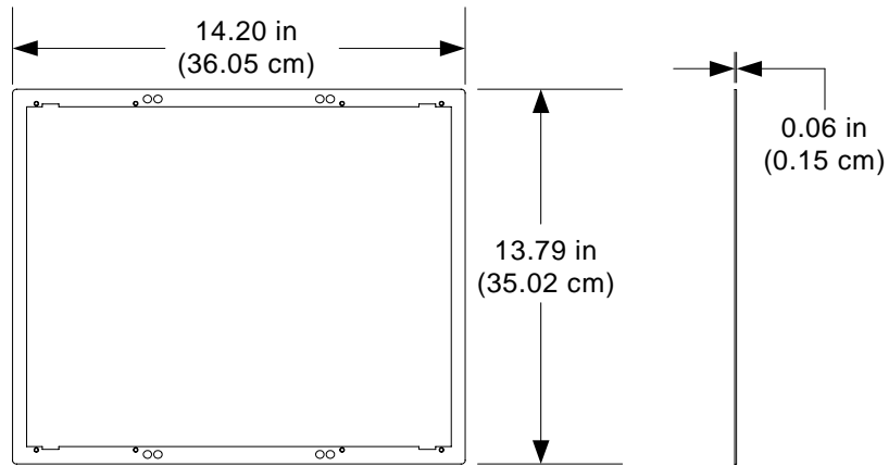
Dimensional Drawing – Mounting Plate
