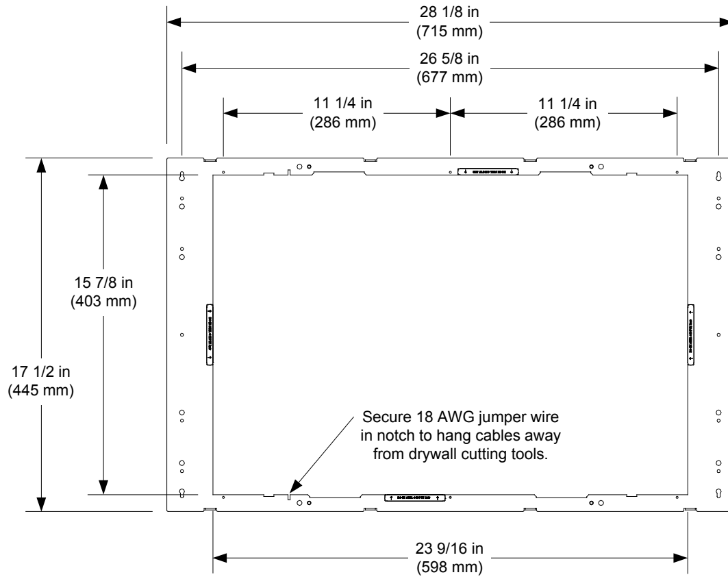
PMK-V24 Overall Dimensions (Front View)
