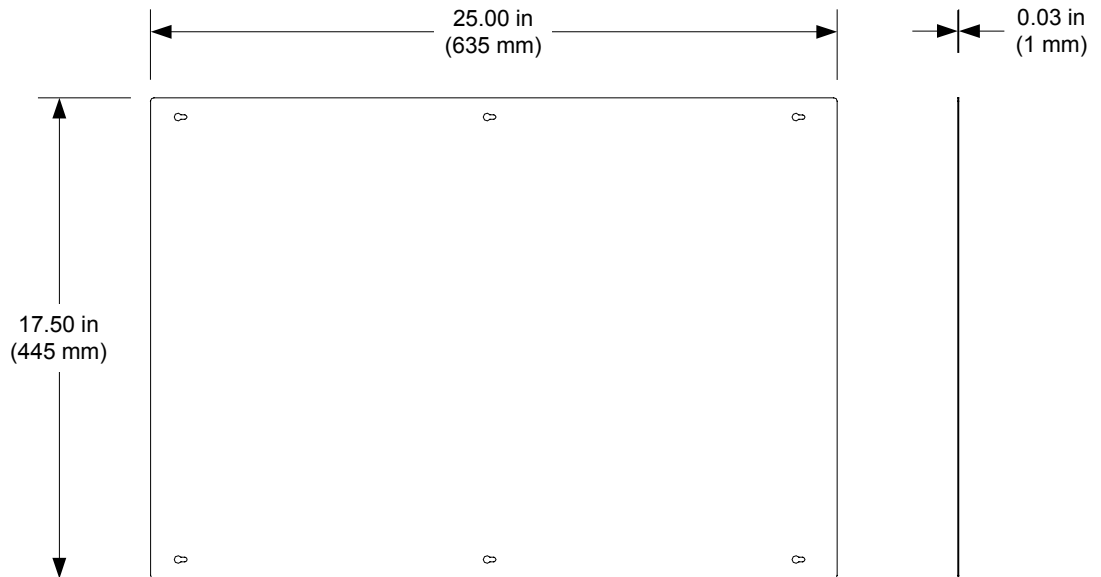
PMK-V24 Overall Dimensions (Cover Plate)
