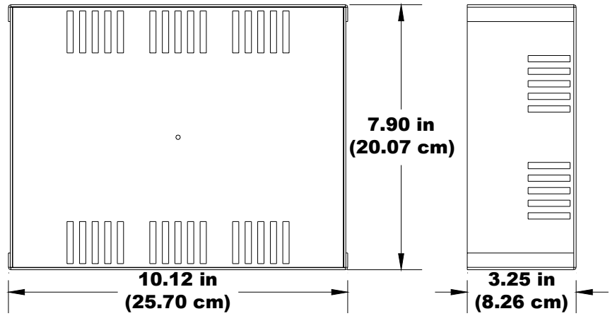
Wall Mount Enclosure
