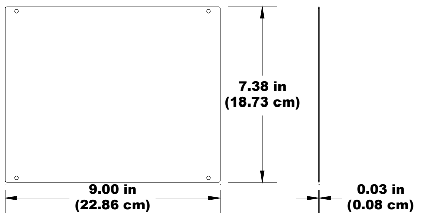
Cover Plate
