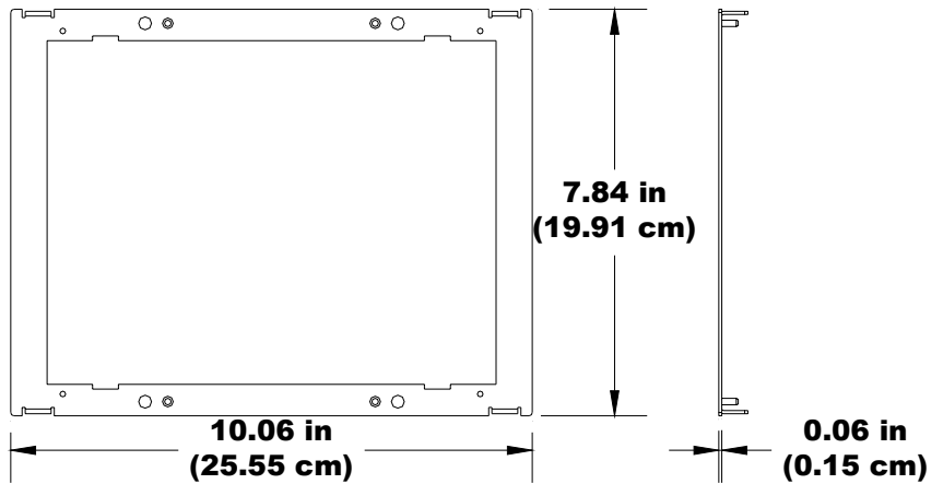
Mounting Plate
