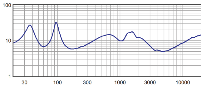
Impedance (Ohms)
