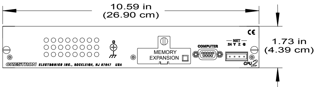
Physical View - Front
