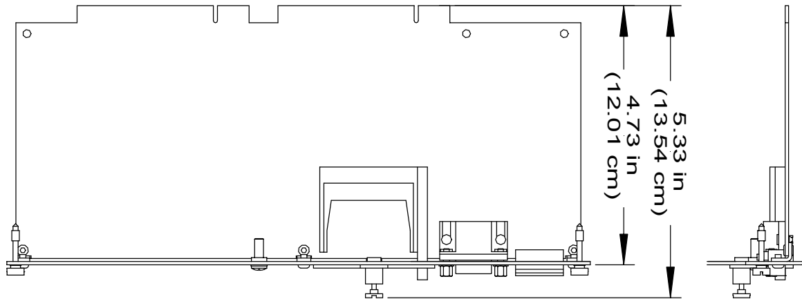
Physical View - Top and Side
