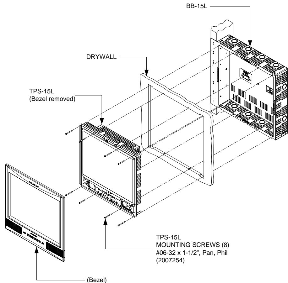
TPS-15L Mounting – Exploded View
