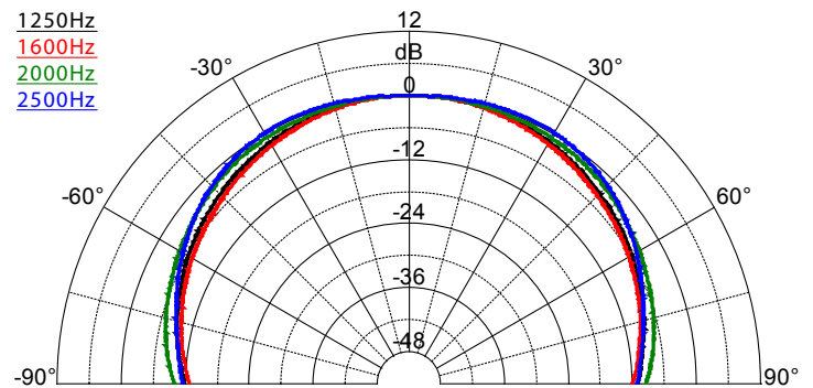
SAROS SR8T – Dispersion Pattern, 1250 Hz - 2500 Hz
