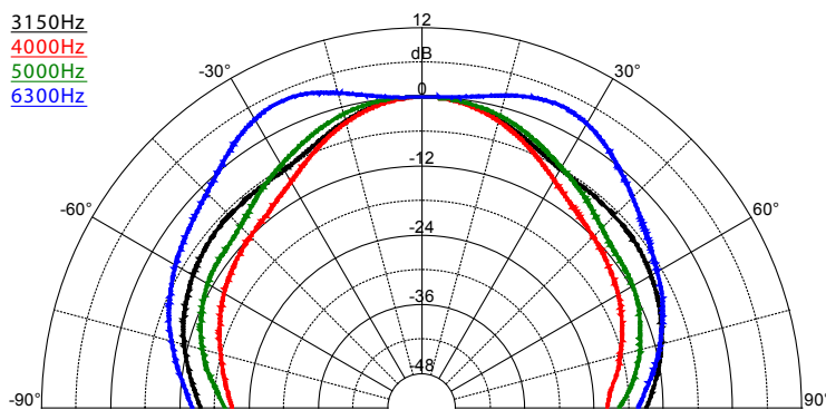
SAROS IC6T – Dispersion Pattern, 3150 Hz - 6300 Hz
