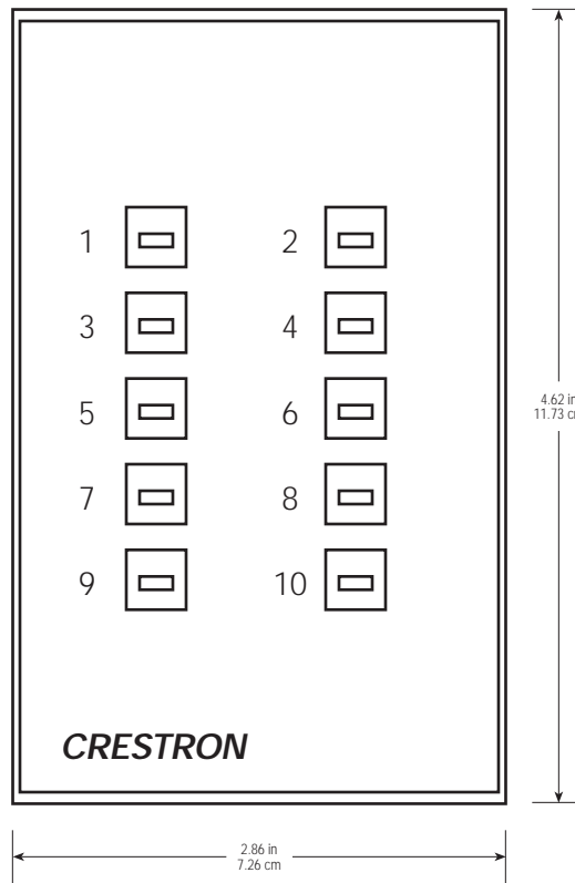
Panel installs in 1-gang electrical box (2.50 in (6.35 cm) minimum depth).
