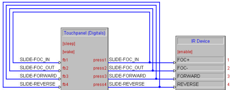
Example Program shown as Block Diagram
