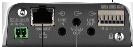
Camera Rear Panel
