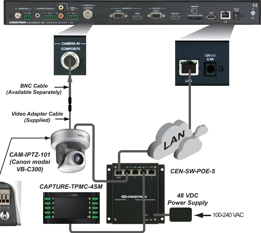
CAPTURE-HD Camera Hookup
