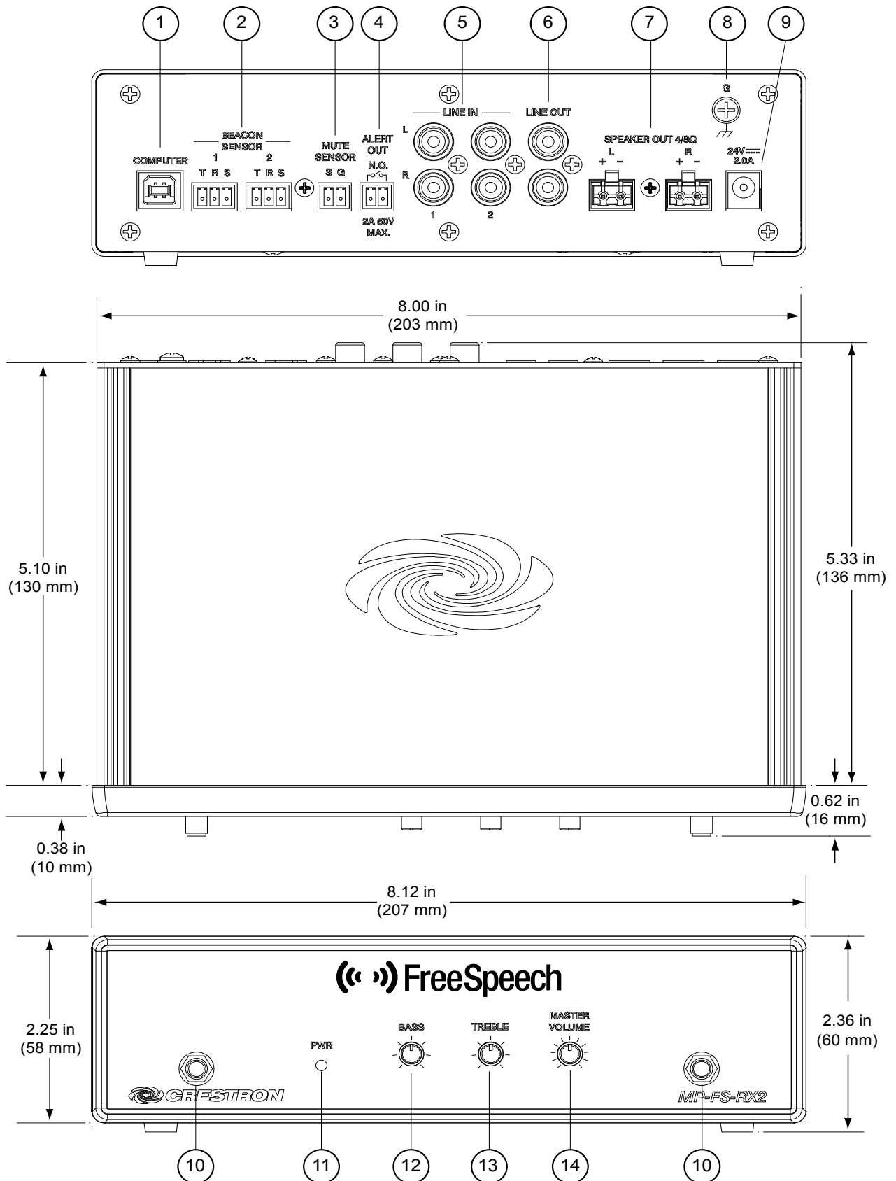
MP-FS-RX1/RX2 Overall Dimensions (MP-FS-RX2 Shown)
