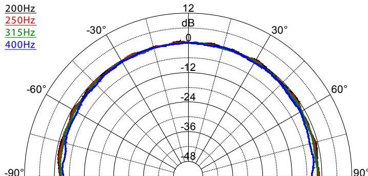
SAROS SR4T – Dispersion Pattern, 200 Hz - 400 Hz
