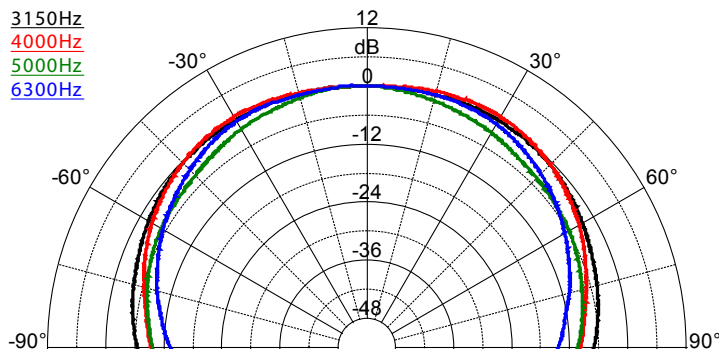
SAROS SR4T – Dispersion Pattern, 3150 Hz - 6300 Hz
