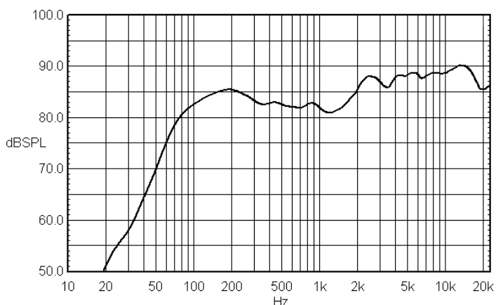
SAROS SR4T – Frequency Response
