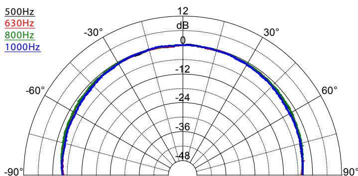
SAROS SR4T – Dispersion Pattern, 500 Hz - 1000 Hz
