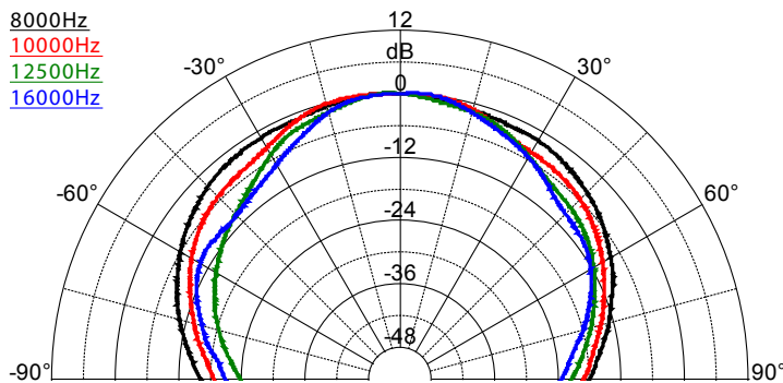
SAROS SR4T – Dispersion Pattern, 8000 Hz - 16000 Hz
