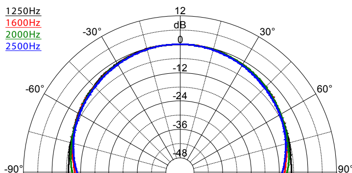
SAROS SR4T – Dispersion Pattern, 1250 Hz - 2500 Hz
