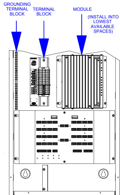
Terminal Block & Module Locations (Double-wide Enclosure)
